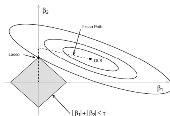
Figure 3: Solution de minimisation duale du Lasso
